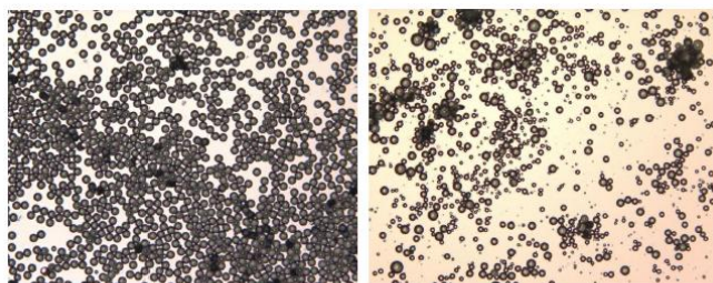
Spheromers® CA 20
